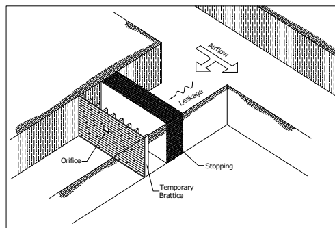
Figure 1: USBM method of measuring single stopping resistance.
