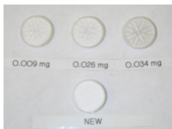
Figure 4. Appearance of full PDM filter after sampling low mass loadings of coal dust.
